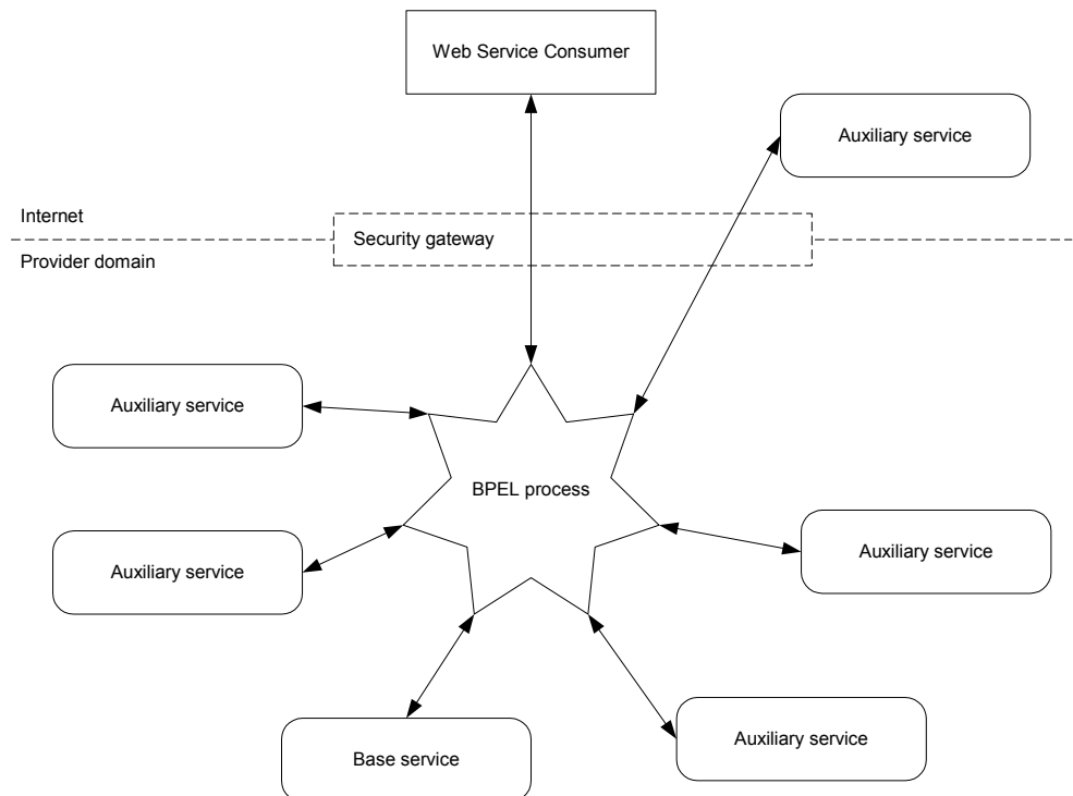
Figure 4-1: Service profiling architecture using BPEL
