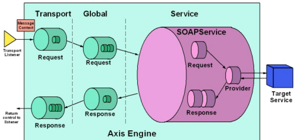
Figure 6-1: Message path in Axis as a server (Axis Architecture Guide [axis])
