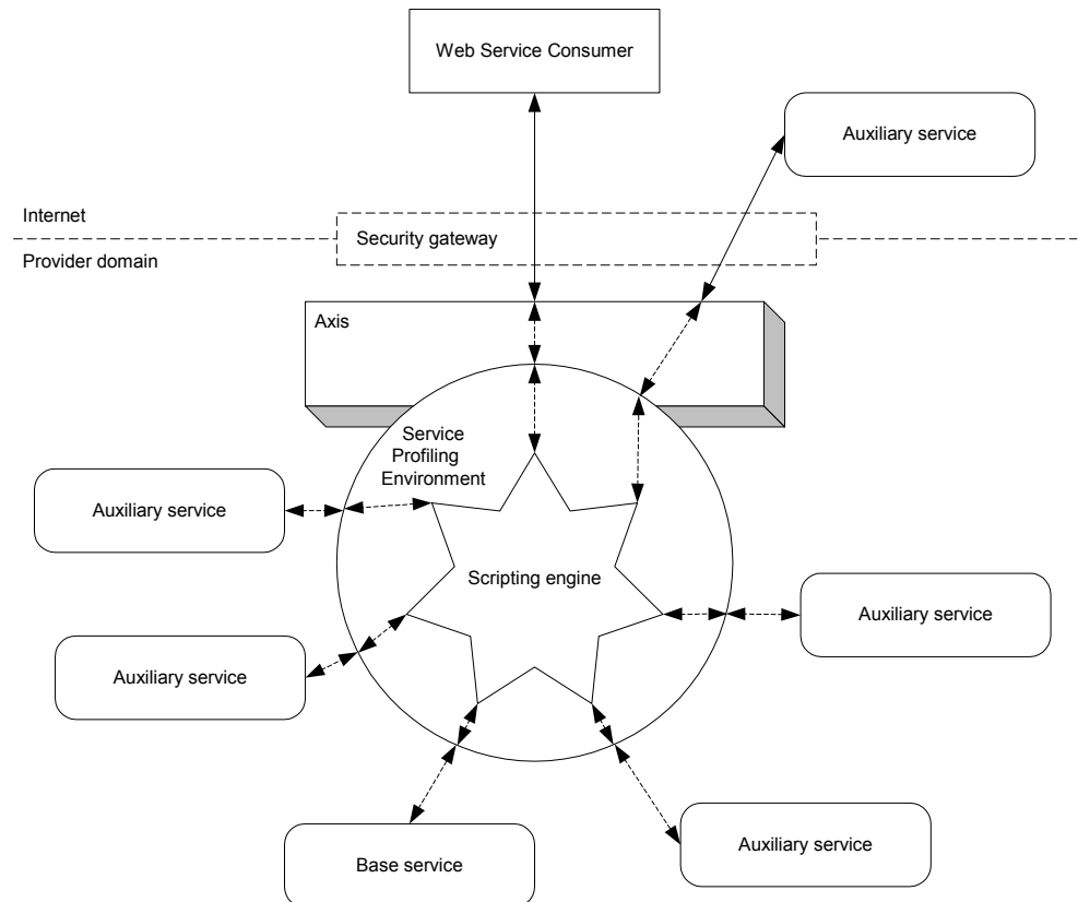
Figure 7-1: Service profiling architecture using a proprietary Java solution
