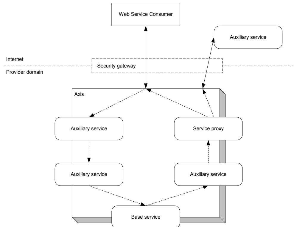
Figure 6-3: Service profiling architecture using Axis handlers
