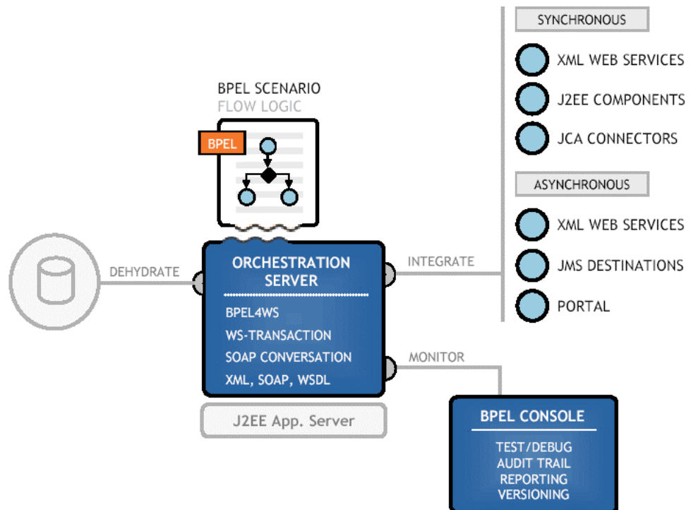
Figure 9-1: Collaxa BPEL server architecture (Collaxa website [collaxa])
