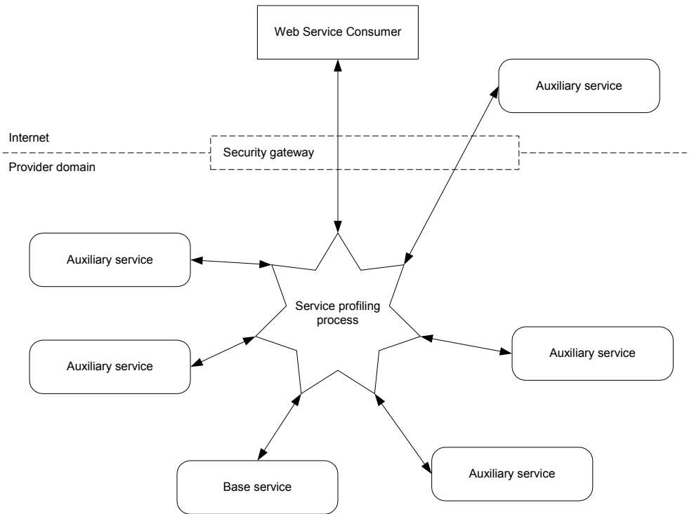
Figure 3-2: General service profiling architecture
