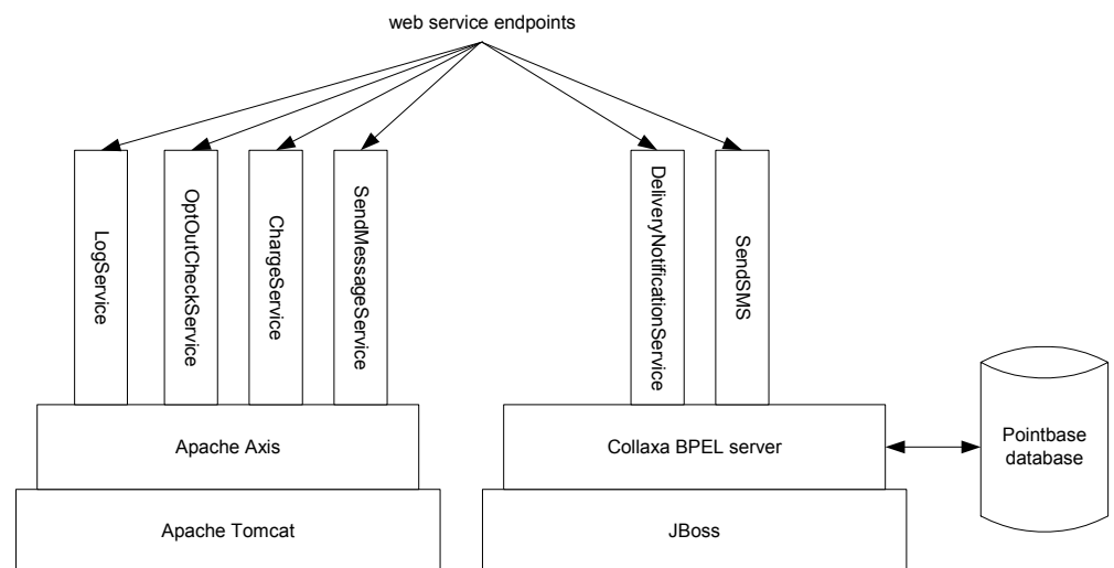
Figure 9-5: Overview of the services in the prototype
