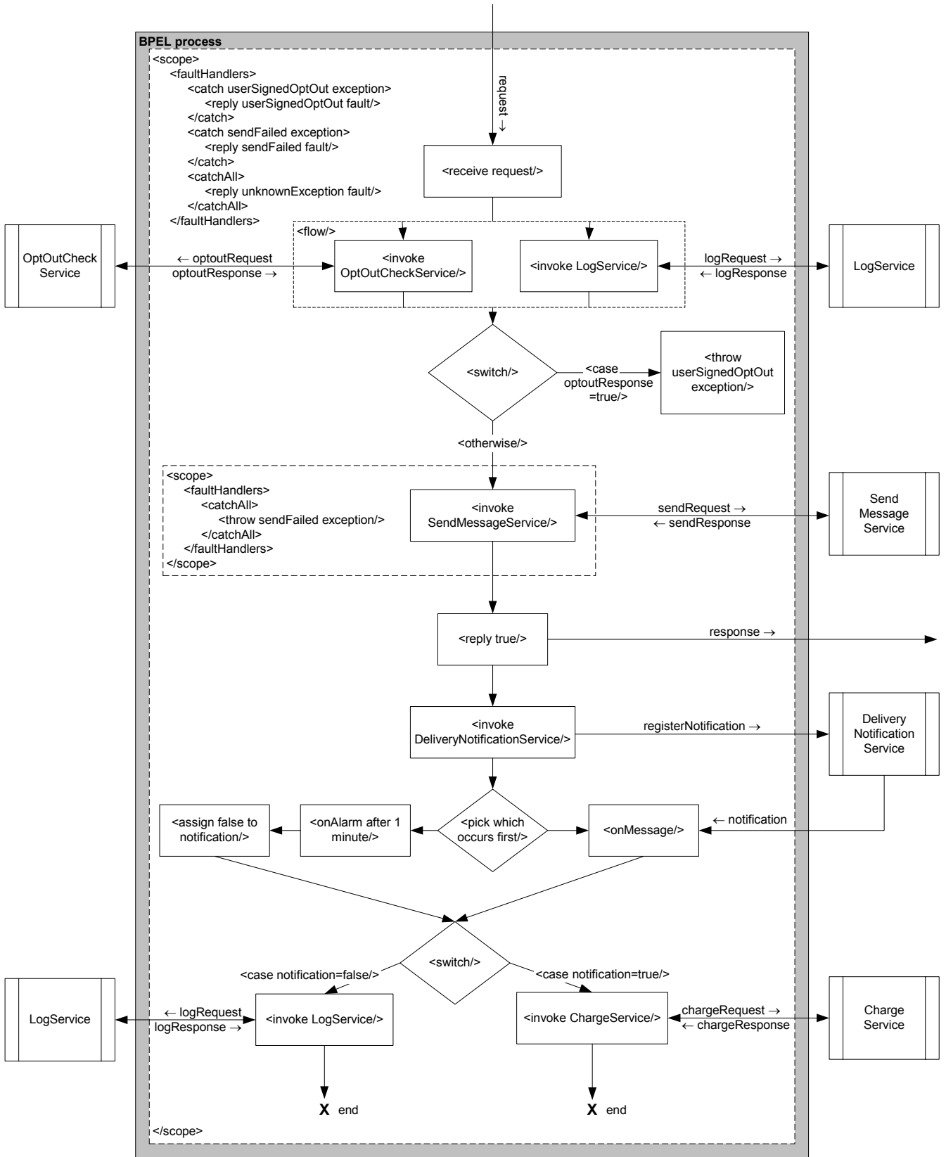
Figure 9-6: Pseudo-flowchart of the SendSMS process that can be mapped to the BPEL source
