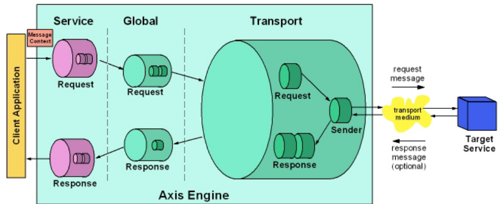
Figure 6-2: Message path in Axis as a client (Axis Architecture Guide [axis])
