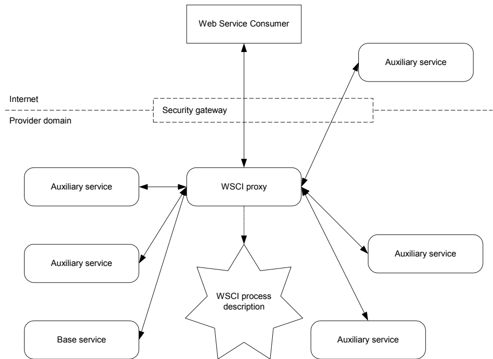
Figure 5-1: Service profiling architecture using WSCI
