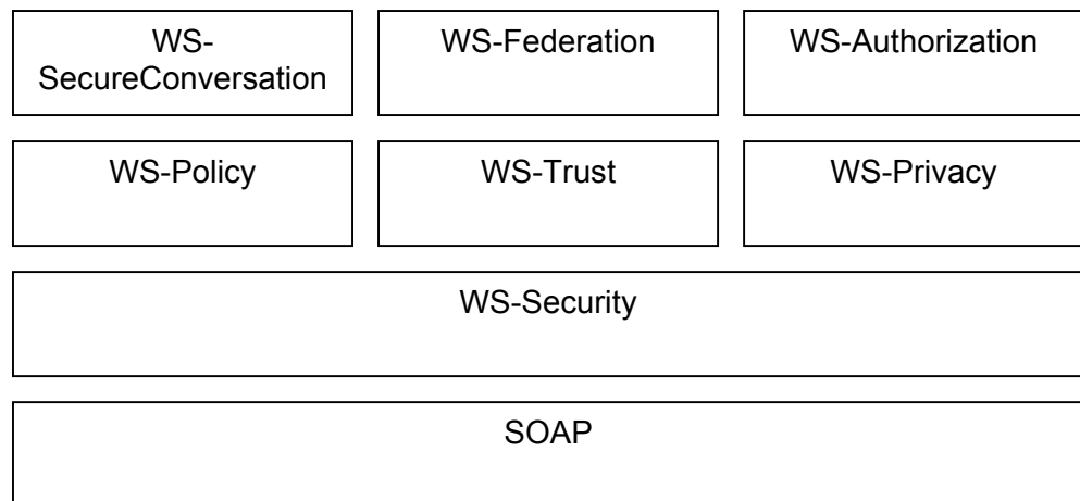
Figure 2-1: WS-Security architecture [della-libera]
