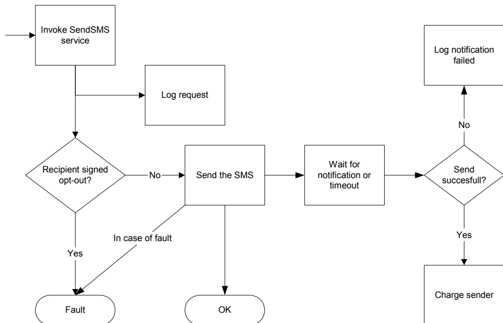
Figure 9-4: Modified version of the flowchart in figure 3-1
