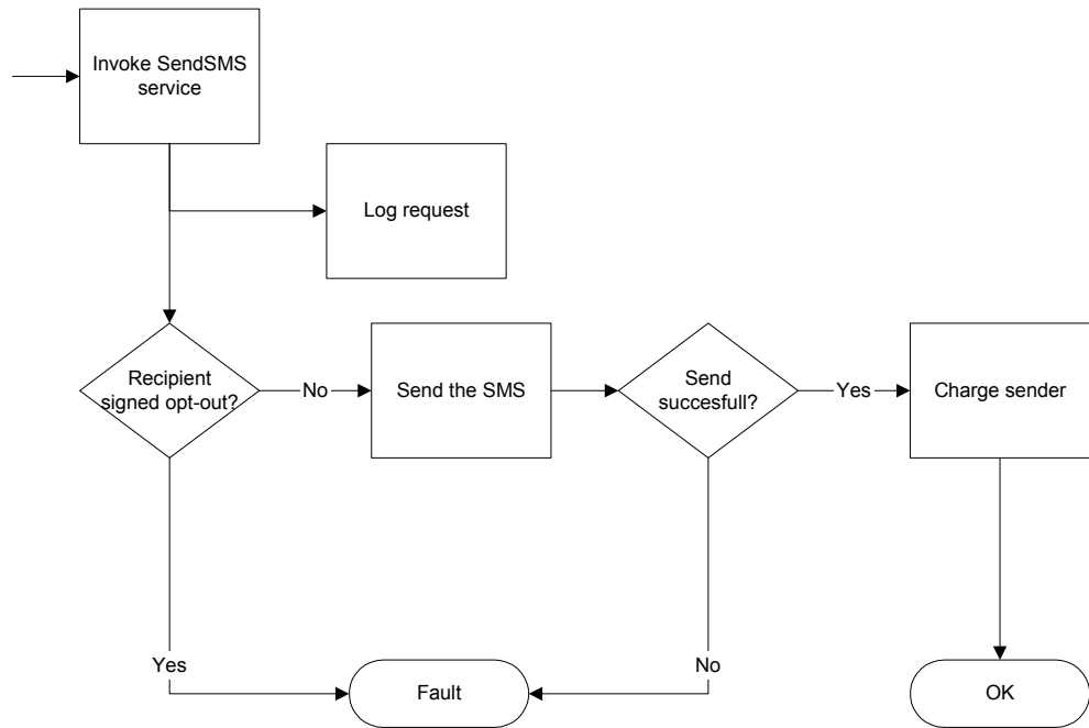
Figure 3-1: Flowchart of an example SendSMS service
